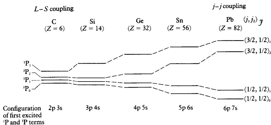
7.10 The splitting of levels in the first excited ^1P and ^3P terms of the carbon sequence.
